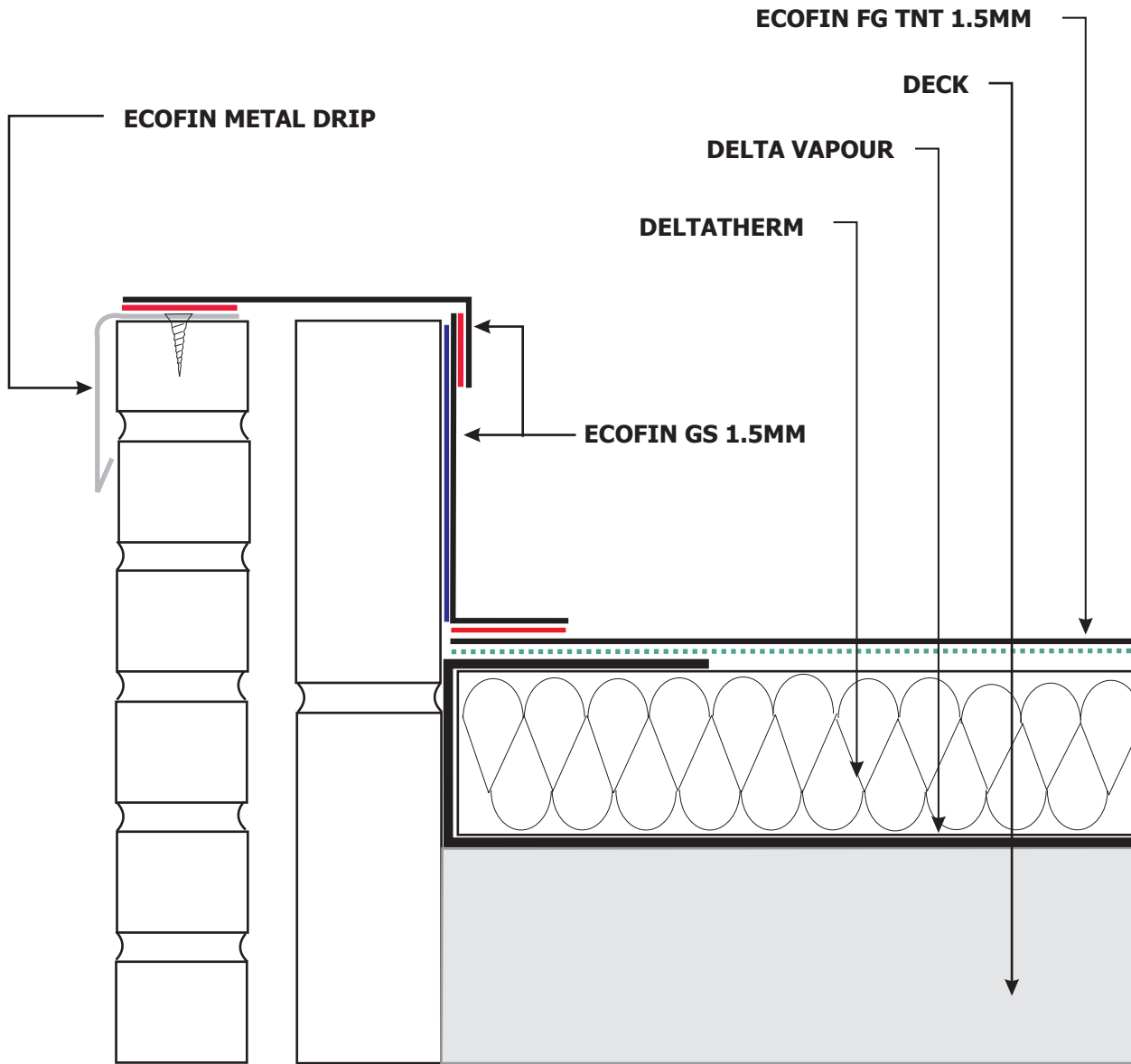
PARAPET DETAIL - FULLY ADHERED
