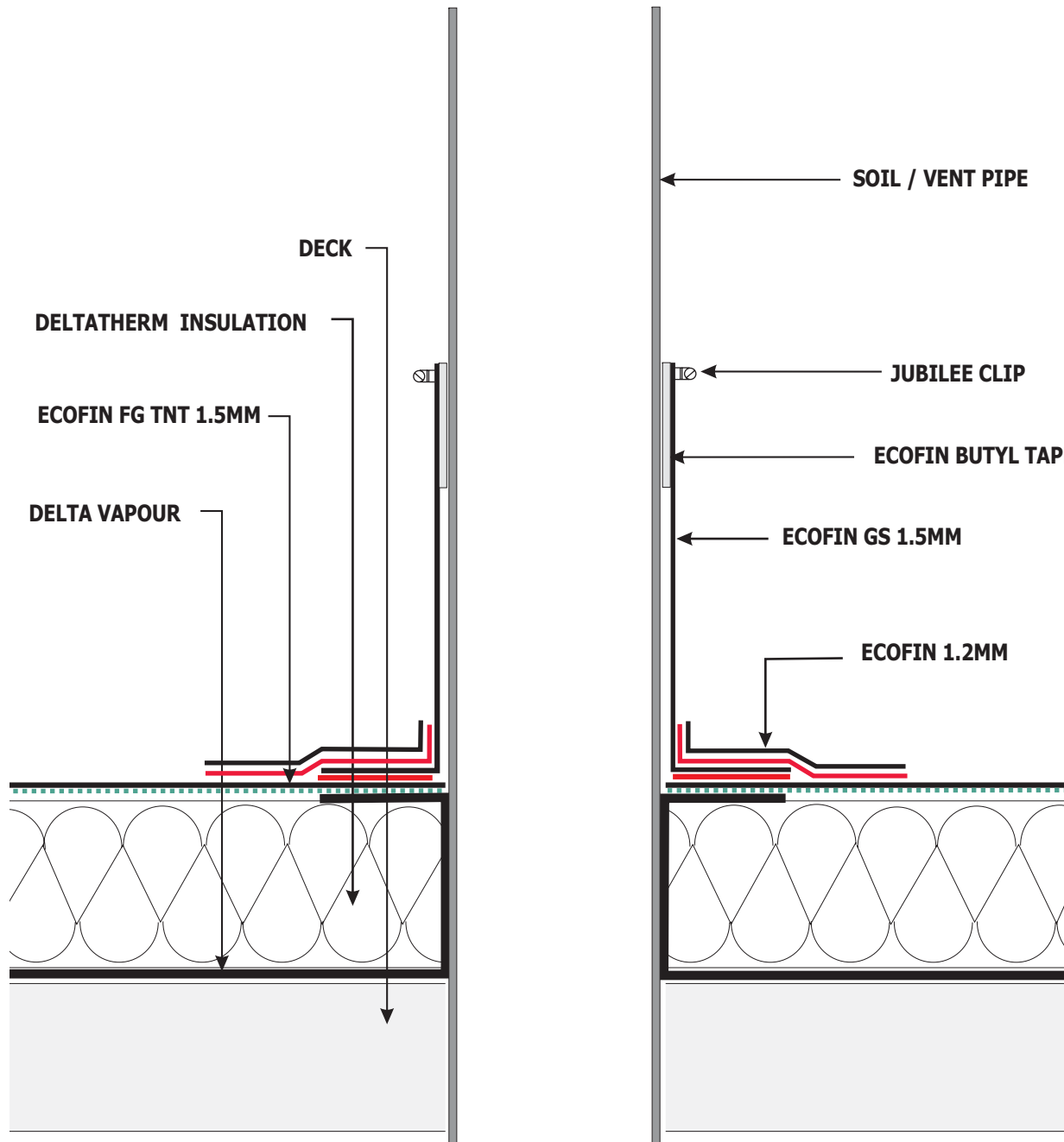
SOIL/VENT PIPE DETAIL
