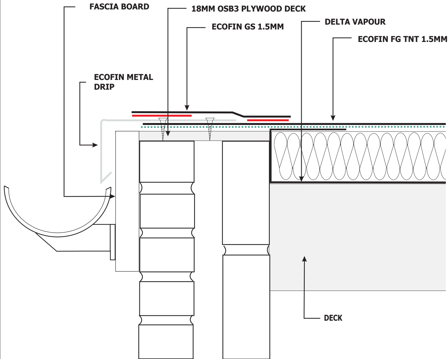
EAVES GUTTER DETAIL - FULLY ADHERED
