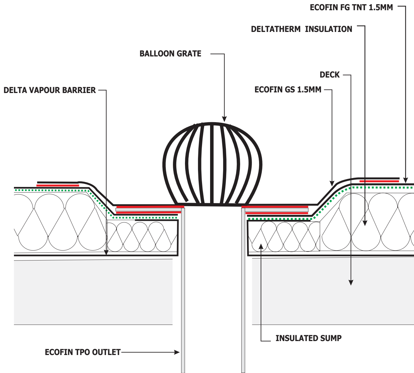
RAINWATER OUTLET DETAIL
