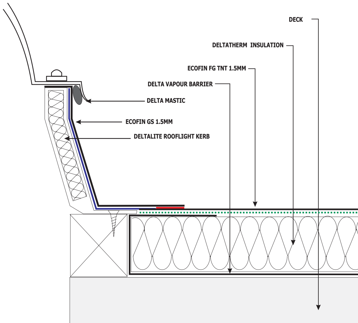
ROOFLIGHT KERB DETAIL
